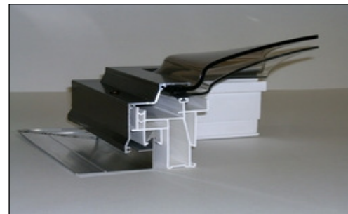
Cross-section of MSF acrylic dome
